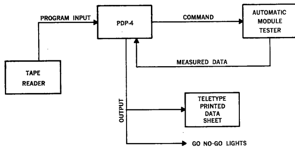
AUTOMATIC MODULE CHECKOUT SYSTEM
